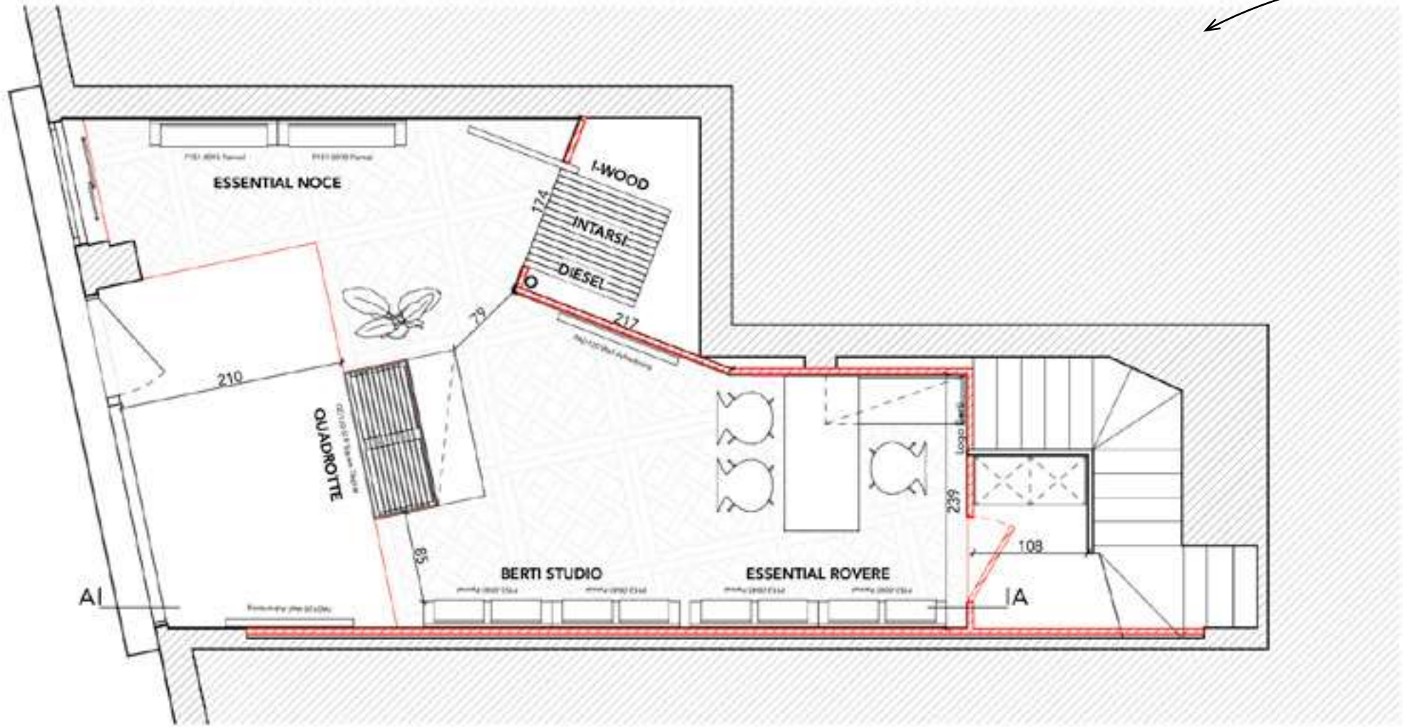
LAYOUT 1:50
